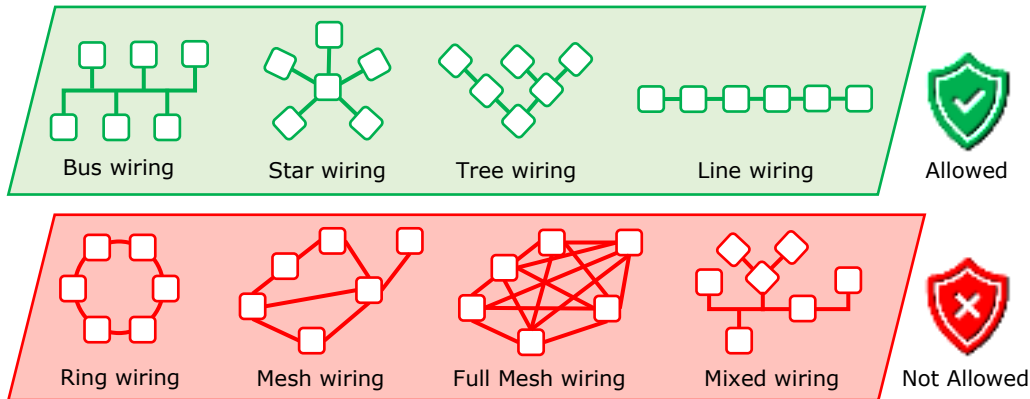
Figure 7: DALI wiring Topologies
