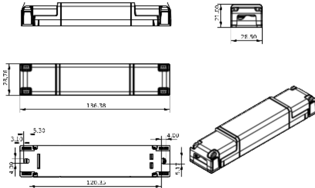
Figure 12: Mechanical dimensions
