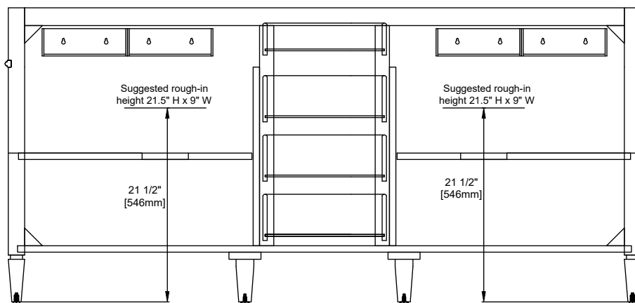
Back View
