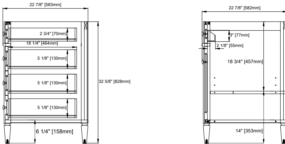
Side View
