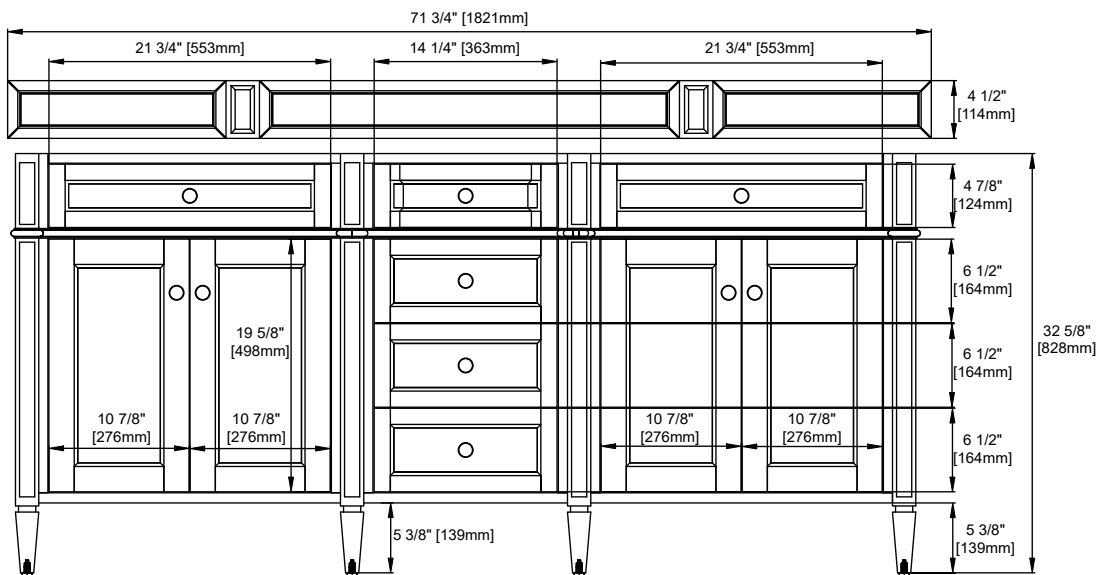
Front View
