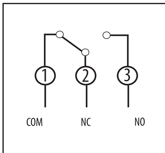
Wiring configuration
