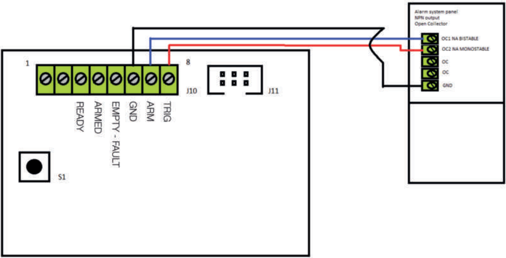
A - UR Fog Modular inputs connected to standard alarm panel outputs
