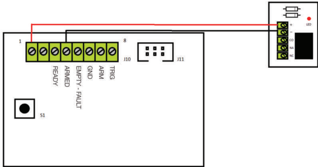
C - Wiring example of UR Fog Modular outputs to drive leds and/or relays
