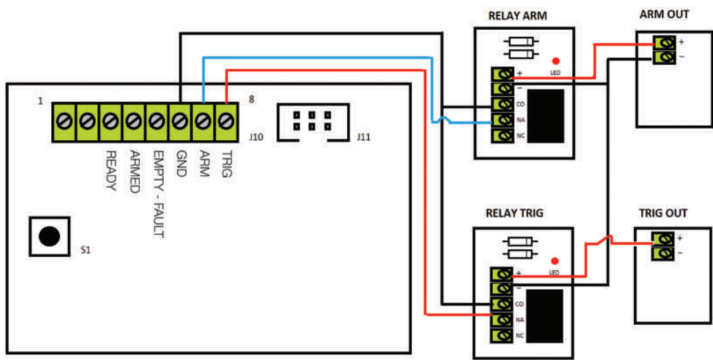
B - UR Fog Modular inputs connected with a clean contact (relays) alarm panel outputs
