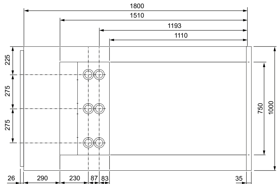
Figure 18 MV Cable Entry with Two Runs
