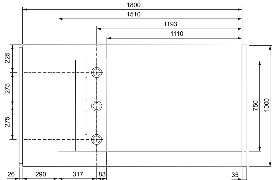
Figure 17 MV Cable Entry with a Single Run
