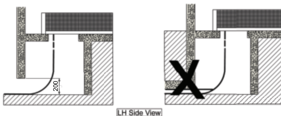
Figure 37 MV Cables Rear Entry
