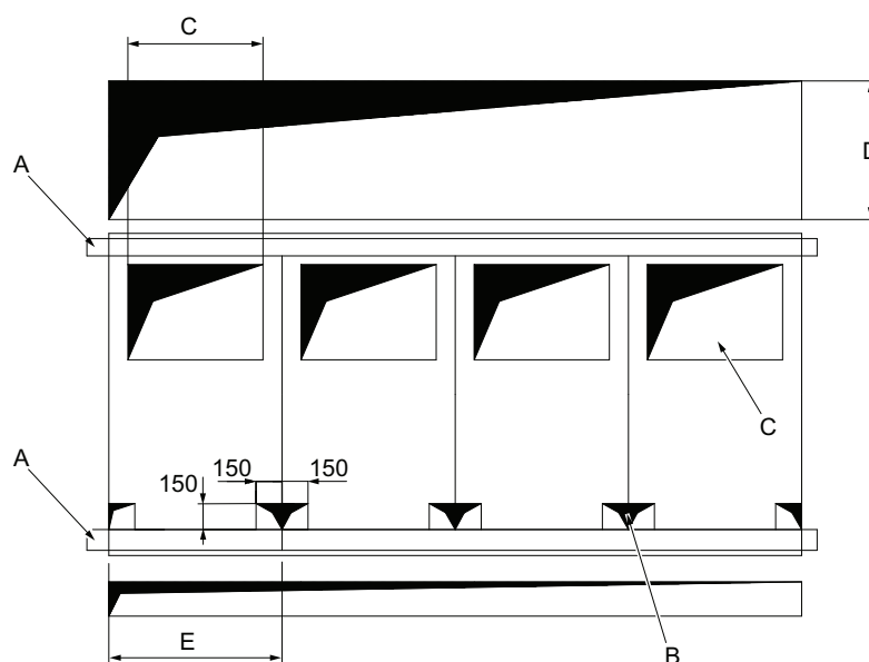
Figure 22 Ground Plan of a MCSeT Switchgear Within a Switchgear Room
