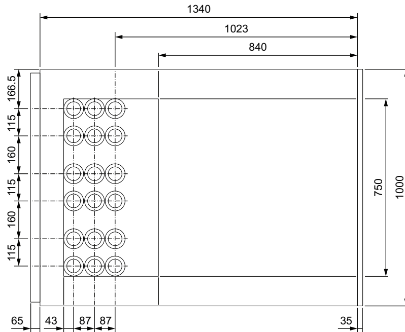
Figure 15 MV Cable Entry with Six Runs
