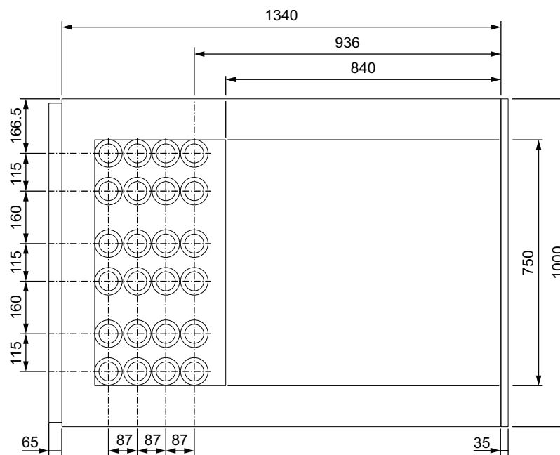
Figure 16 MV Cable Entry with Eight Runs
