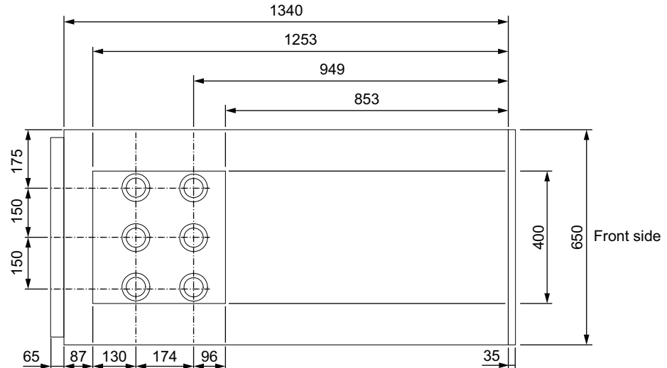
Figure 9 MV Cable Entry with Two Runs
