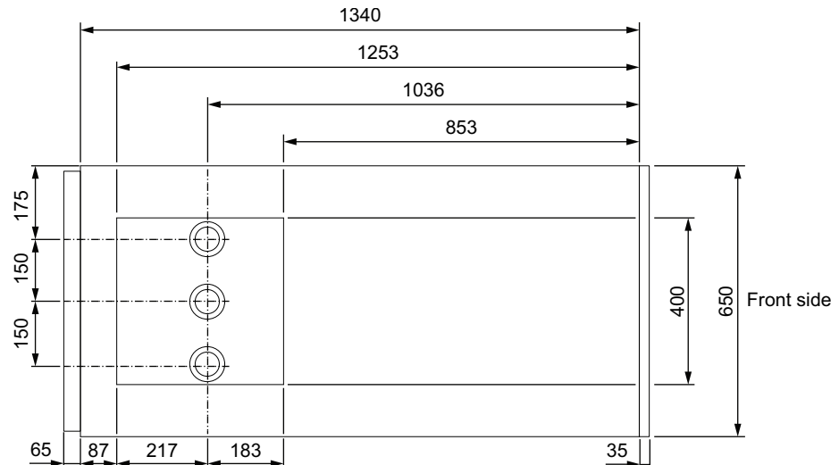
Figure 8 MV Cable Entry with a Single Run
