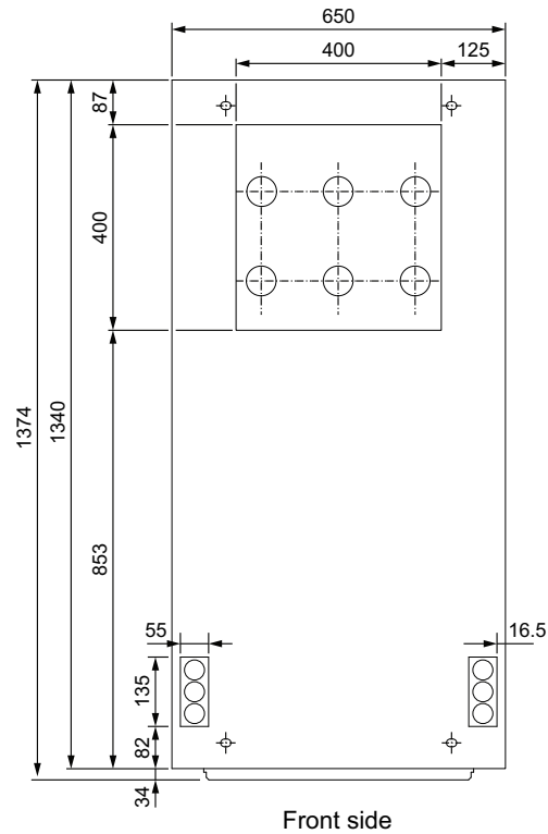
Figure 23 Bottom Plate of 650 mm Cubicle
