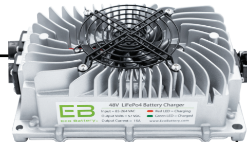
BATTERY CHARGER
