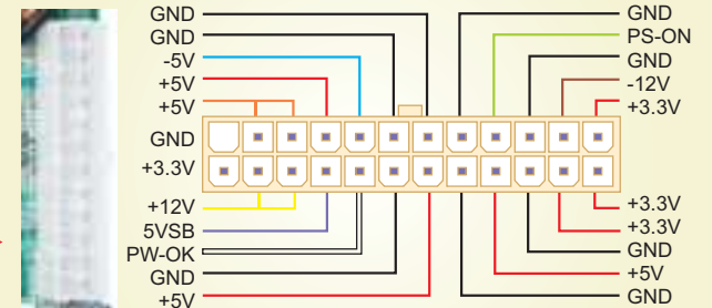
Power Connector
