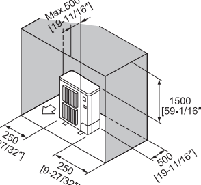
Fig. 12-2-7 Obstacles at rear, sides and above only
