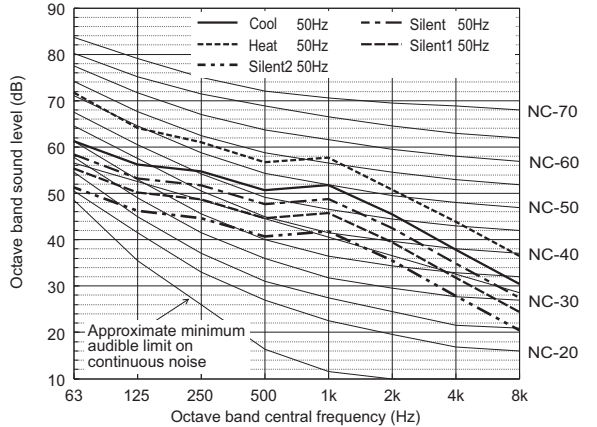
Sound level of PUMY-P250YBM2
