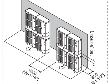
Fig. 12-2-13 Stacked groups arrangement
