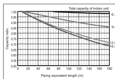
Fig.4 Correction of refrigerant piping length *1
