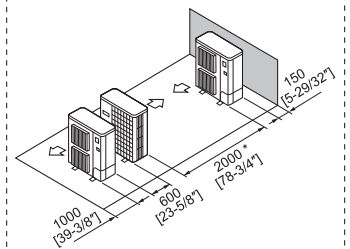
Fig. 12-2-11 Parallel individuals arrangement
