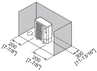
Fig. 12-2-4 Obstacles at rear and sides only
