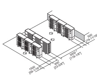
Fig. 12-2-12 Parallel groups arrangement
