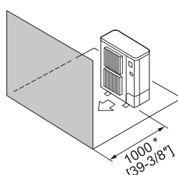
Fig. 12-2-5 Obstacles at front only
