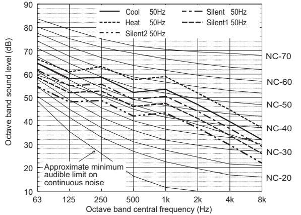
Sound level of PUMY-P300YBM2
