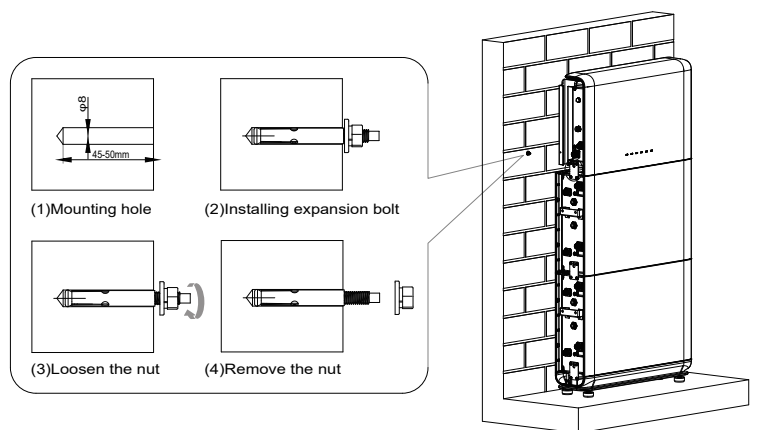
Figure.3-7 Expansion bolts installation
