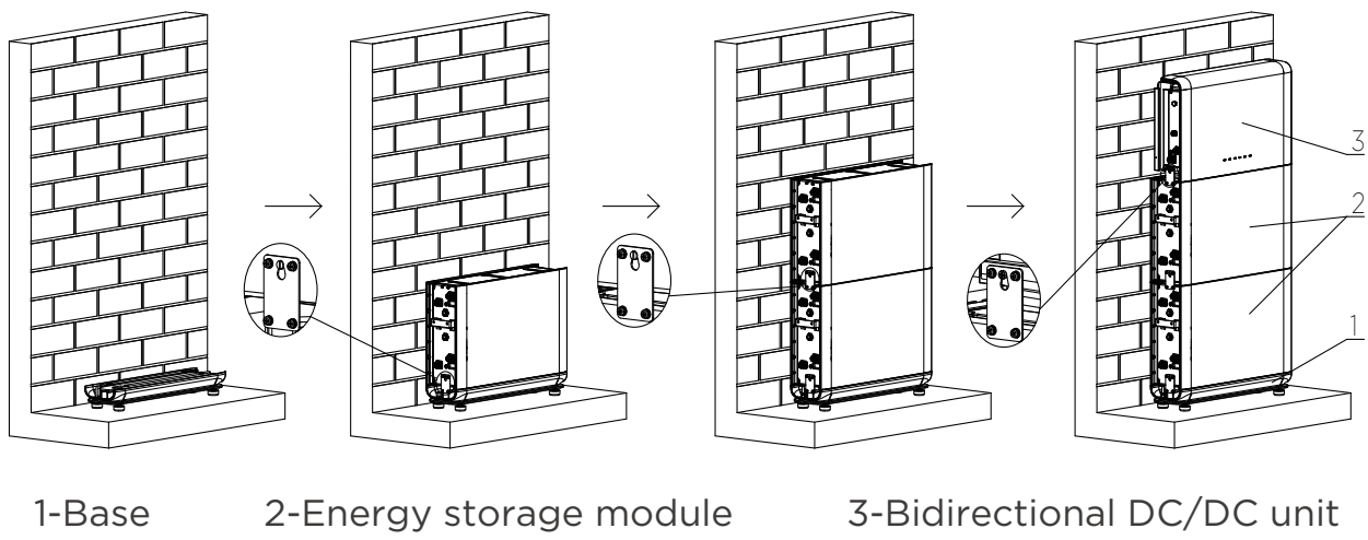
1-Base 2-Energy storage module 3-Bidirectional DC/DC unit Figure.3-5 Installing the energy storage and bidirectional DC/DC unit diagram
