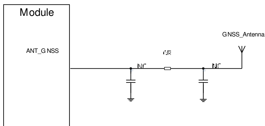
Figure 4-3-1 GNSS passive antenna reference circuit
