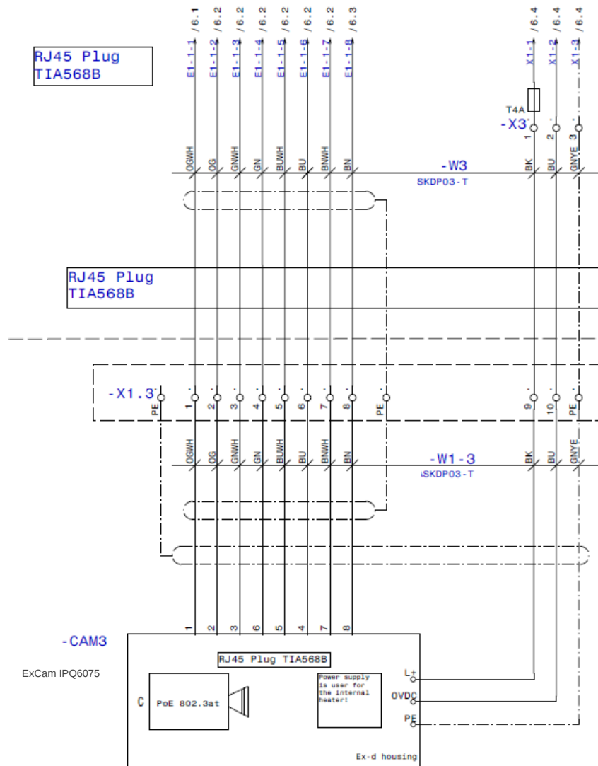
Fig. 5-5 Sample circuit of terminal box EXTB-3 (model LL)
