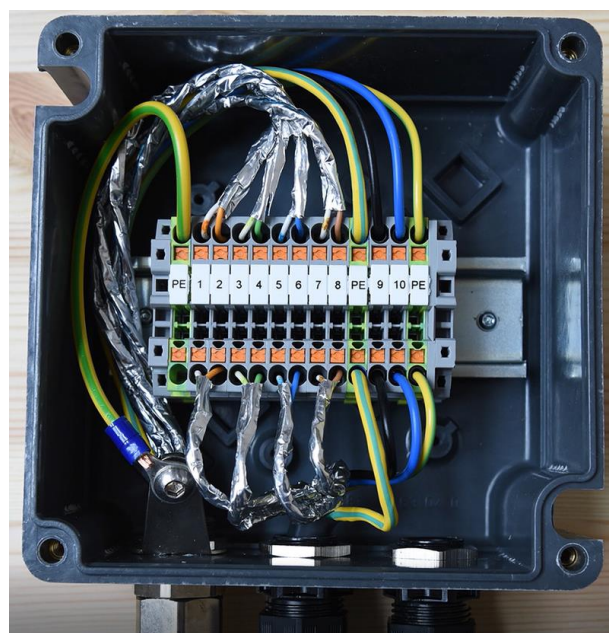
Fig. 5-6 Photo of the occupied terminal box EXTB-3
