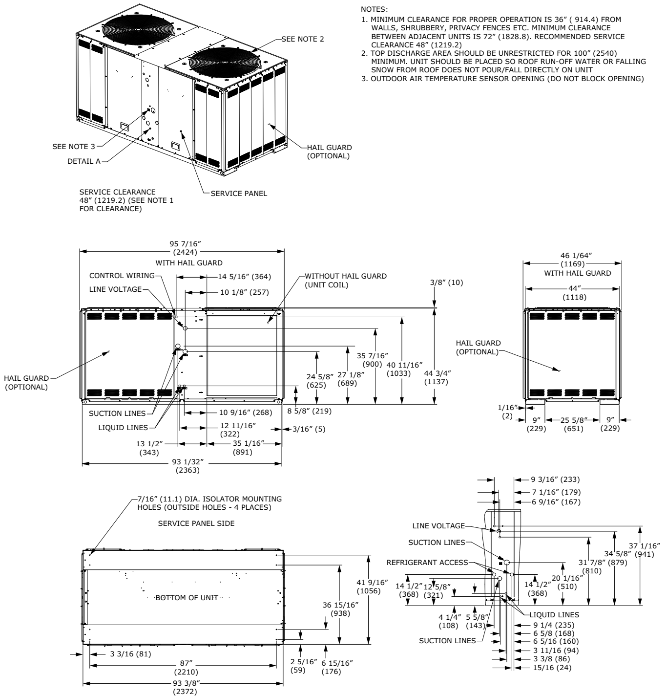
Figure 13. 13, 16.7 ton condensing, dual compressor – in (mm)
