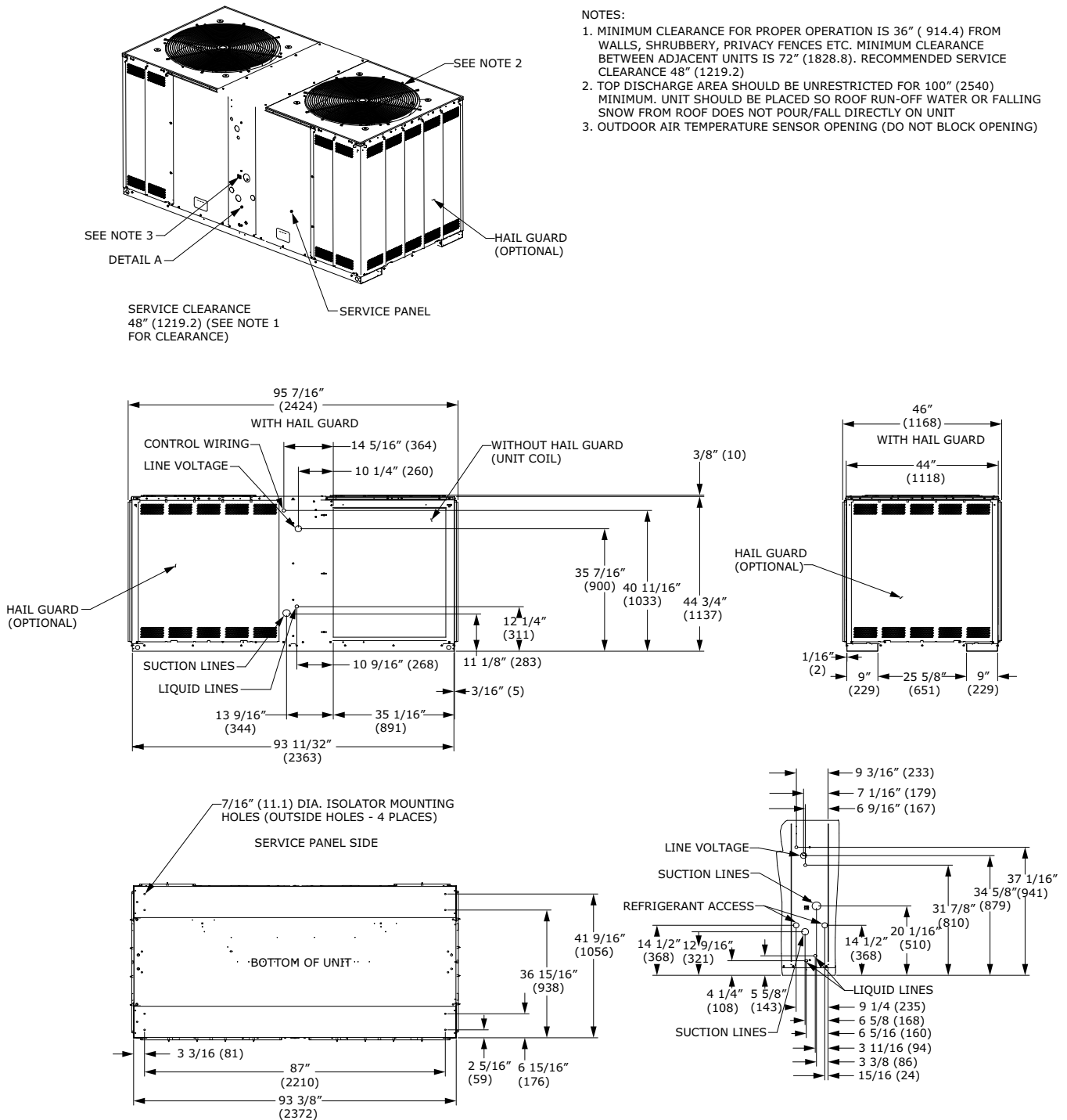
Figure 14. 13, 16.7 ton condensing, manifolded compressor – in (mm)
