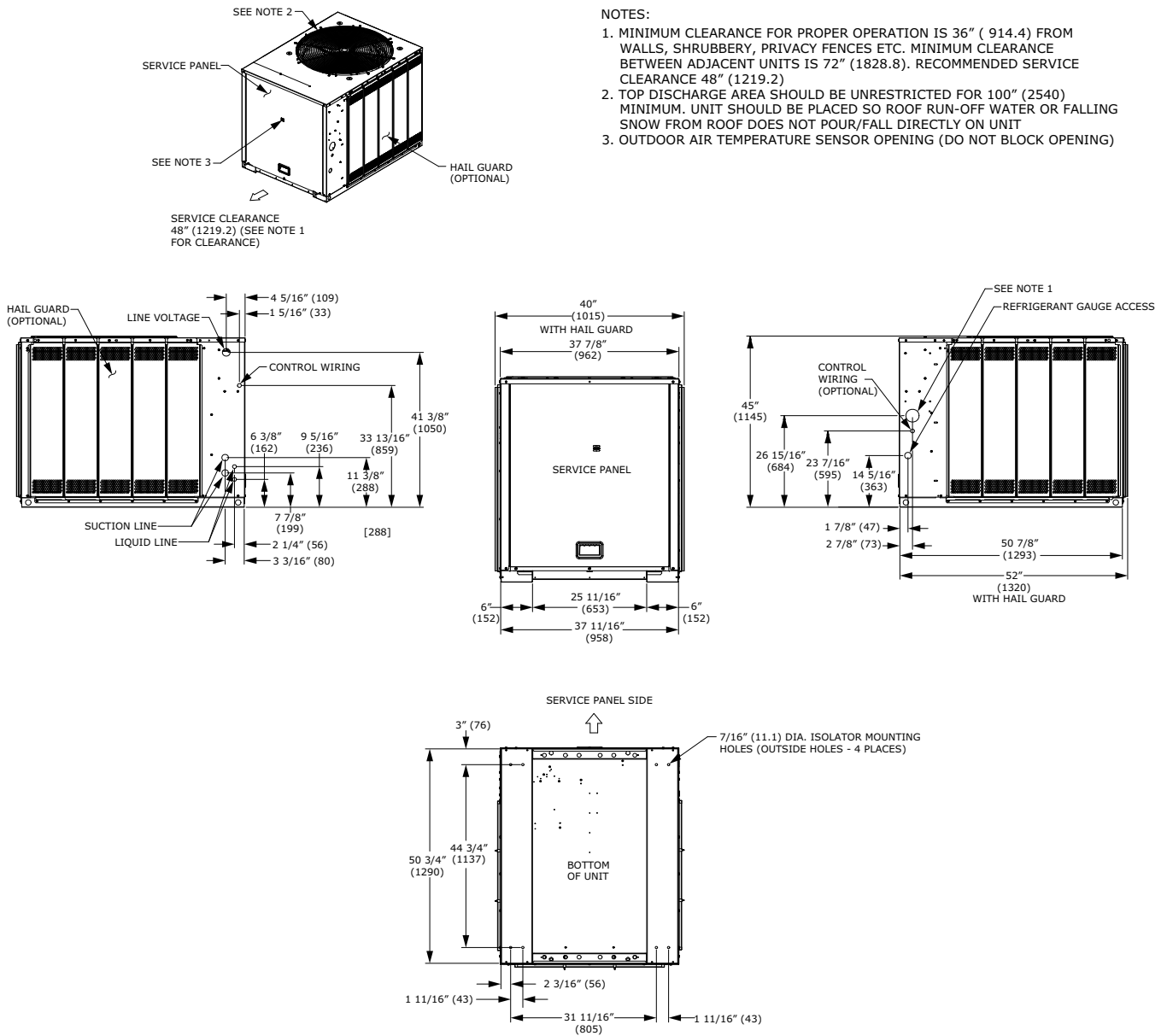
Figure 12. 10.4 ton condensing, dual compressor – in (mm)
