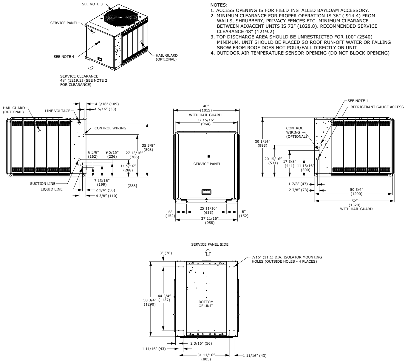
Figure 11. 8.33 ton condensing, dual compressor – in (mm)
