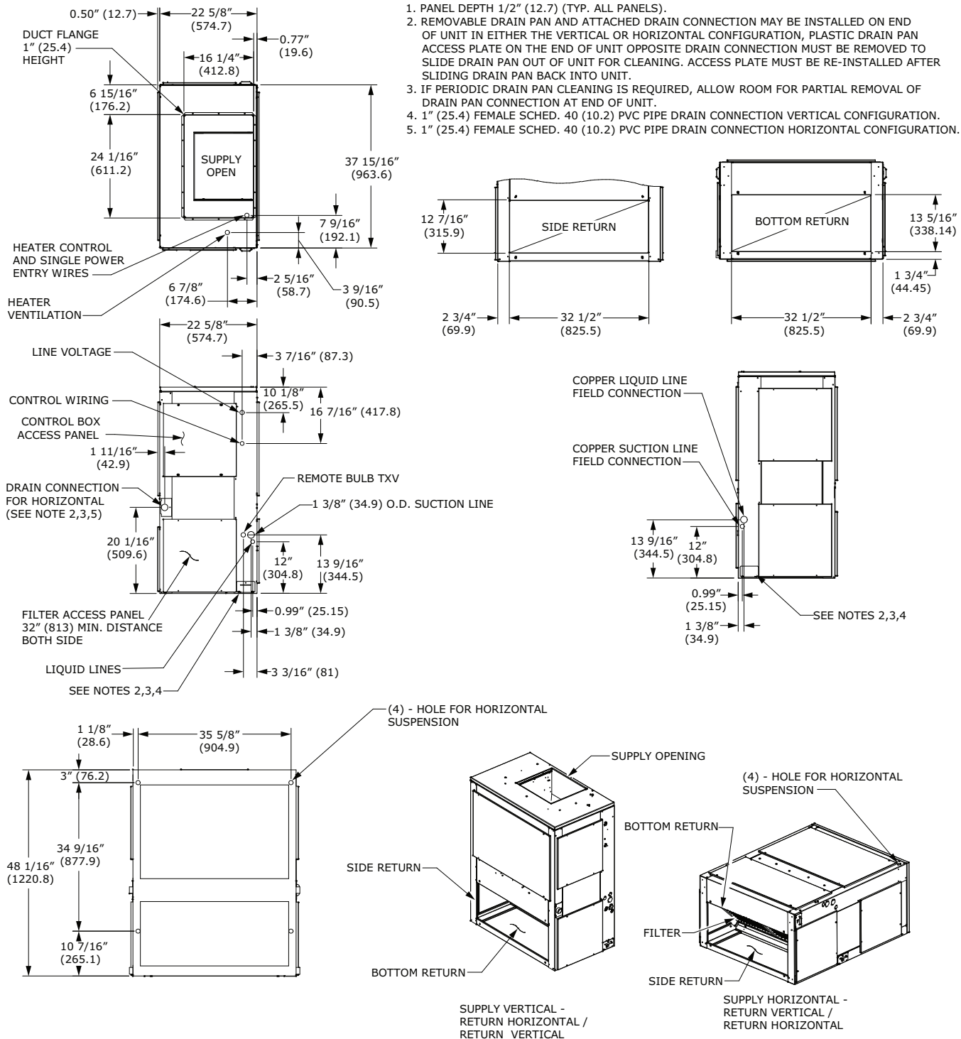
Figure 16. 4.6 ton air handler, single circuit – in (mm)
