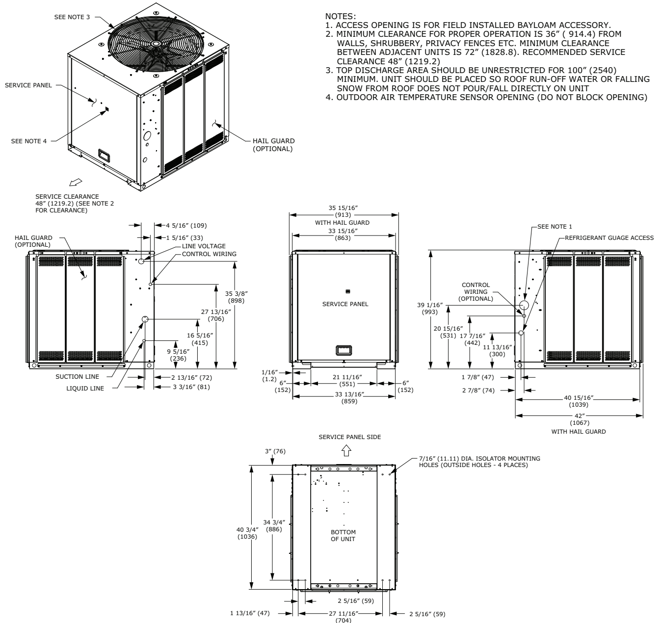
Figure 8. 5, 6.25 ton condensing, single compressor – in (mm)
