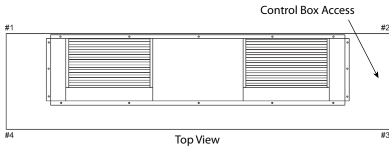
Figure 35. Horizontal — TWE051, 072, 076, 101
