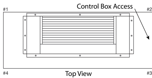
Figure 34. Vertical — TWE126, 156, 201, 251
