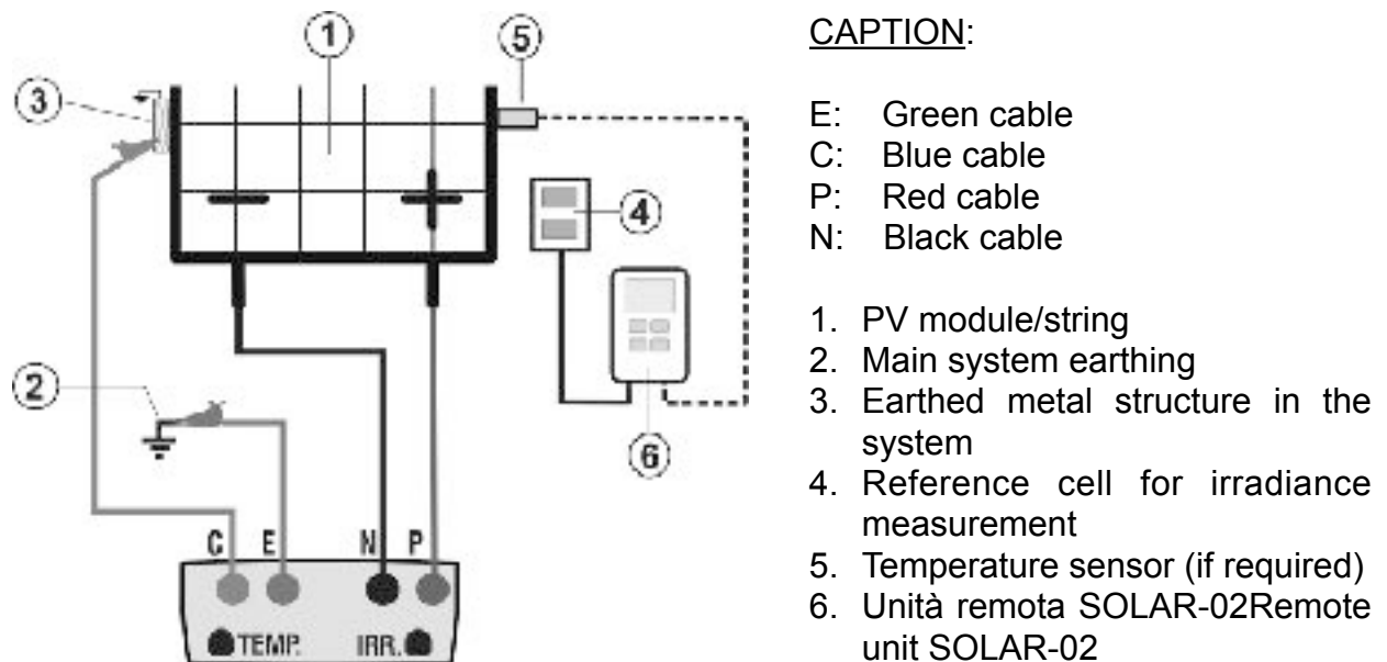
Fig. 8: Connection for IVCK test with direct irradiance measurement
