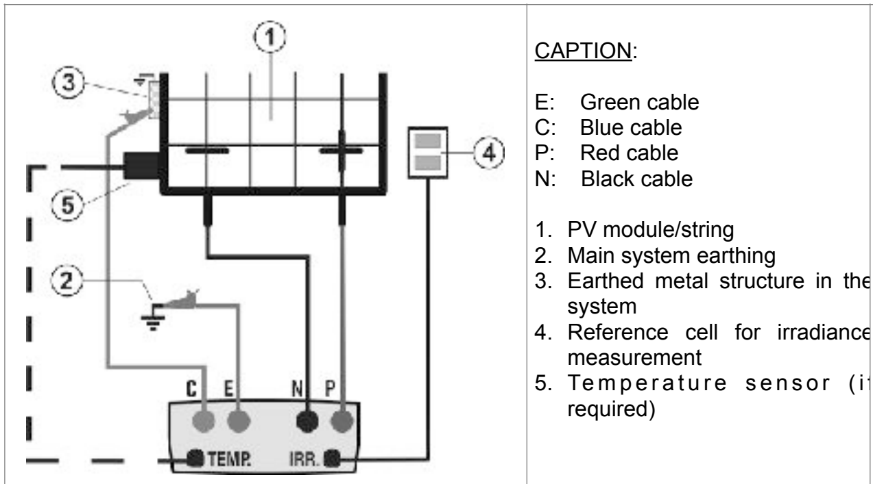
Fig. 8: Connection for IVCK test with direct irradiance measurement
