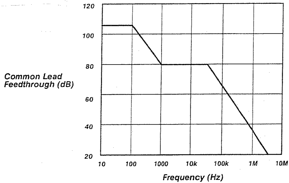
Figure 1-3: Common-lead feedthrough characteristics
