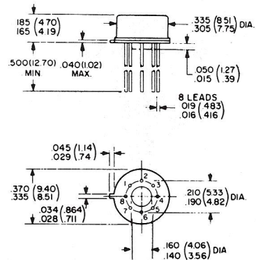
DIMENSIONAL OUTLINE
