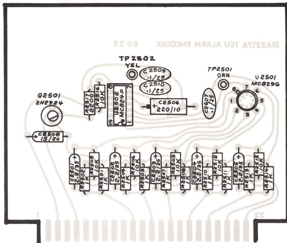
Figure 37. TCU Alarm Encoder (Board 25), Parts Location
