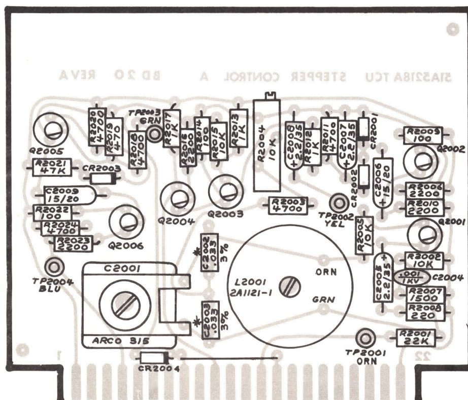
Figure 38. TCU Stepper Control A (Board 20), Parts Location
