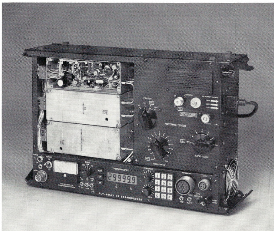
Internal view of TW100F showing modules (one with cover removed).
