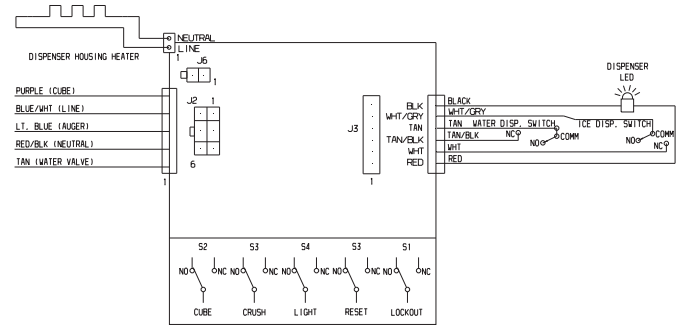
ICE & WATER CONTROL BOARD
