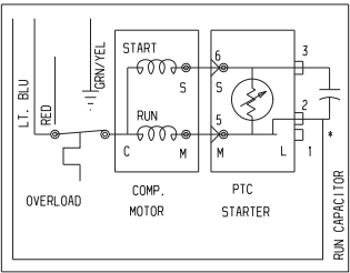
P.T.C. STARTER WITH RUN CAPACITOR
