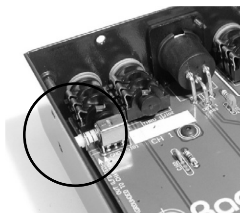
Fig. 3 Channel 1 side access switch connects chassis ground to pin-1. Factory set 'out' to 'float'
