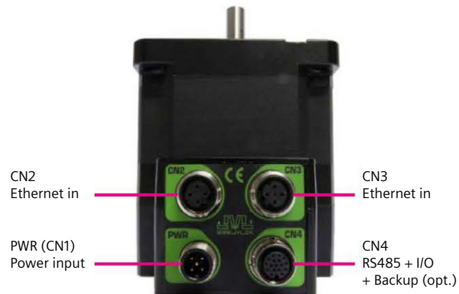
Figure 30: Interface and Connections for Smart Motor
