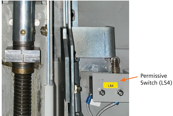
Figure 3: Racking mechanism with LS4 position switch shown
