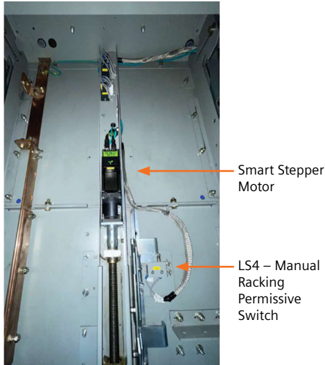
Figure 15: Racking Mechanism for HMI Setup
