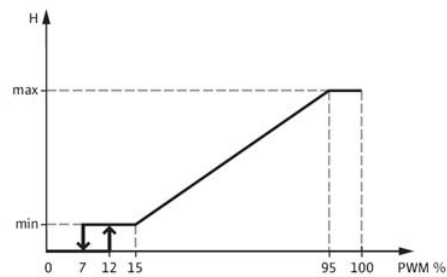
PWM signal logic (solar):
