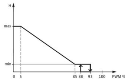
PWM signal logic (heating):
