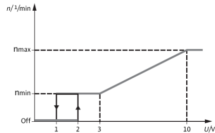
PWM(0-10V) signal logic
