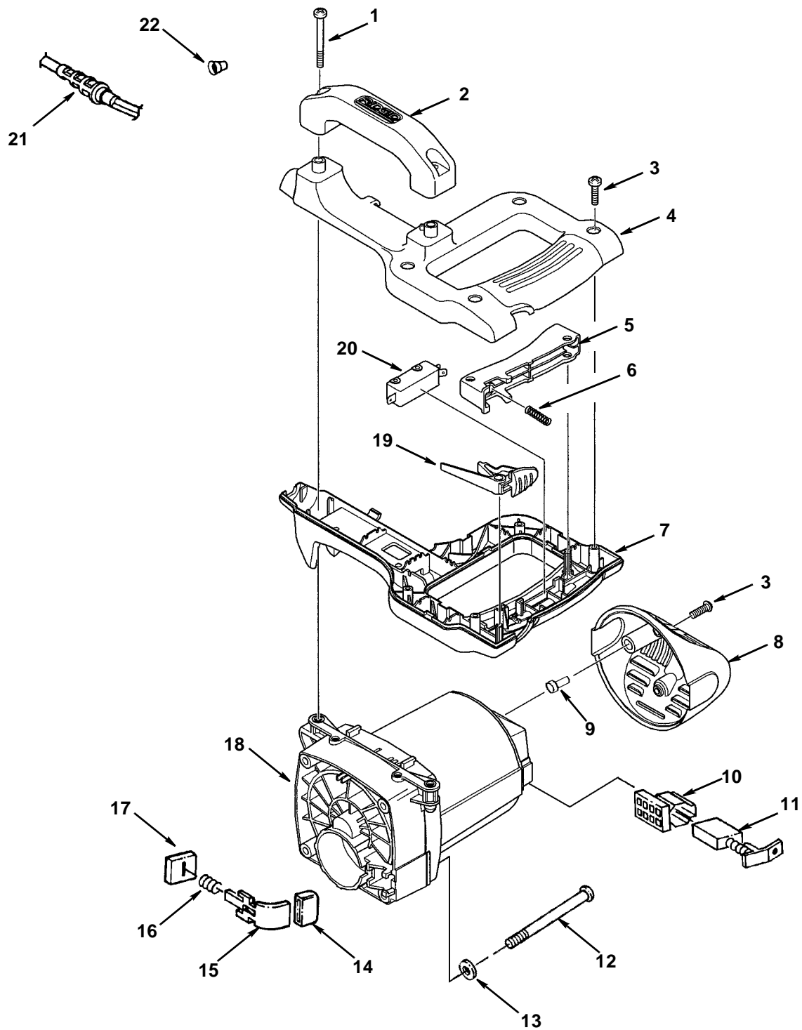
Figure 2 - Motor Assembly
