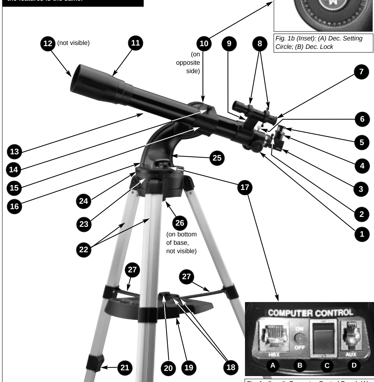
Fig. 1: DS-2000 Series Telescope.
