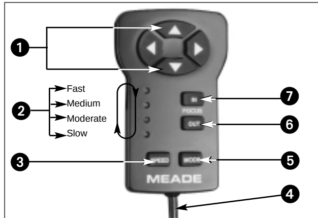
Fig. 33: Electronic Controller. (1) Arrow Keys; (2) Indicator Lights; (3) SPEED Key; (4) Coil Cord; (5) MODE Key; (6) OUT Key; (7) IN Key.
