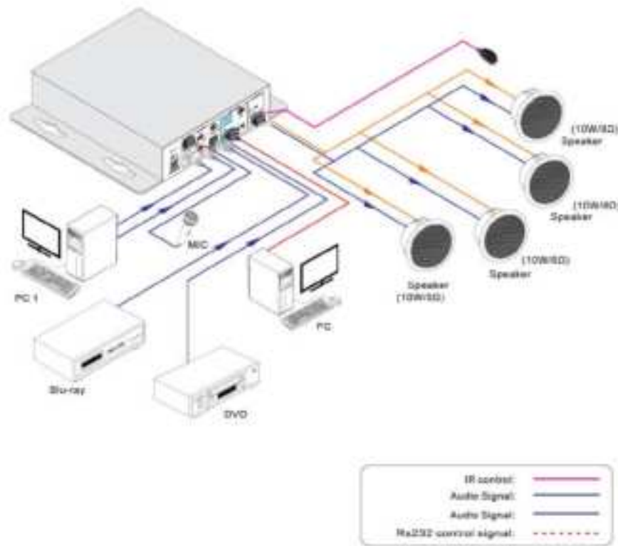
Figure 3 System Diagram
