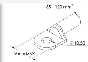
(*)Cable lugs
