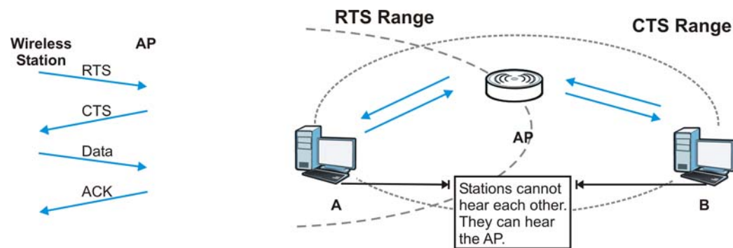
Figure 107 RTS/CTS
