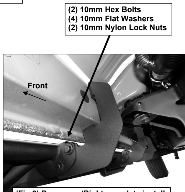
(Fig 9) Passenger/Right complete install
