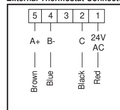
2-Way Communication External Thermostat Connector
