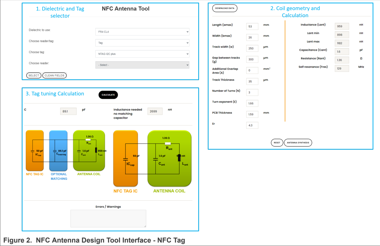
Figure 2 shows the NFC Tag Antenna and tuning calculation part.
