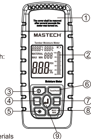
MS6900 Diagram
