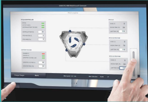
Two-Hand Operation
