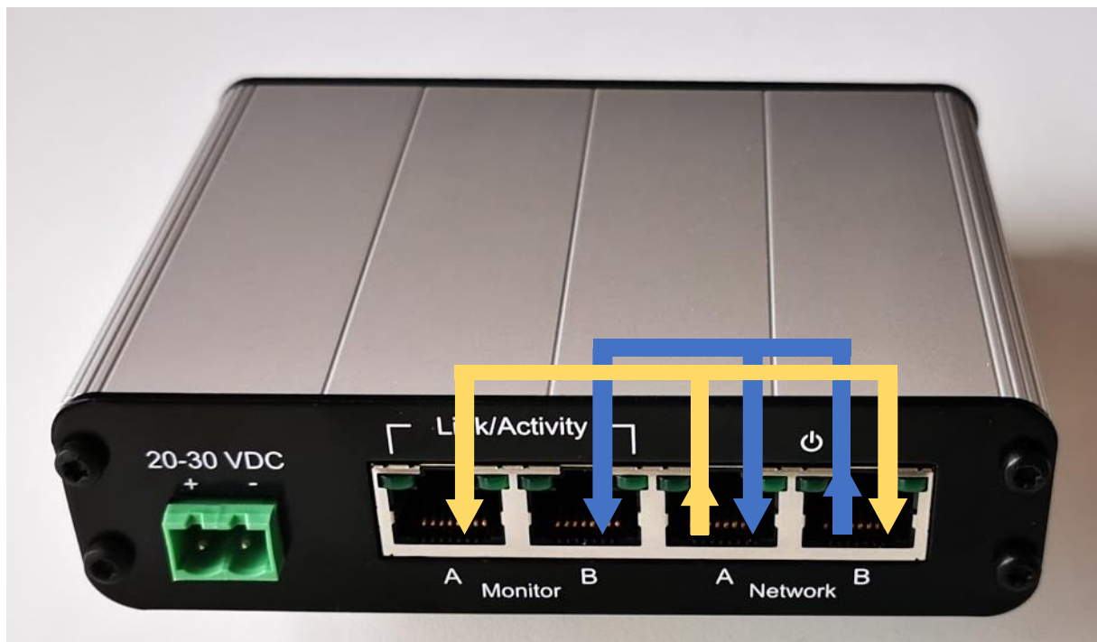
Figure 1 - Internal connections
