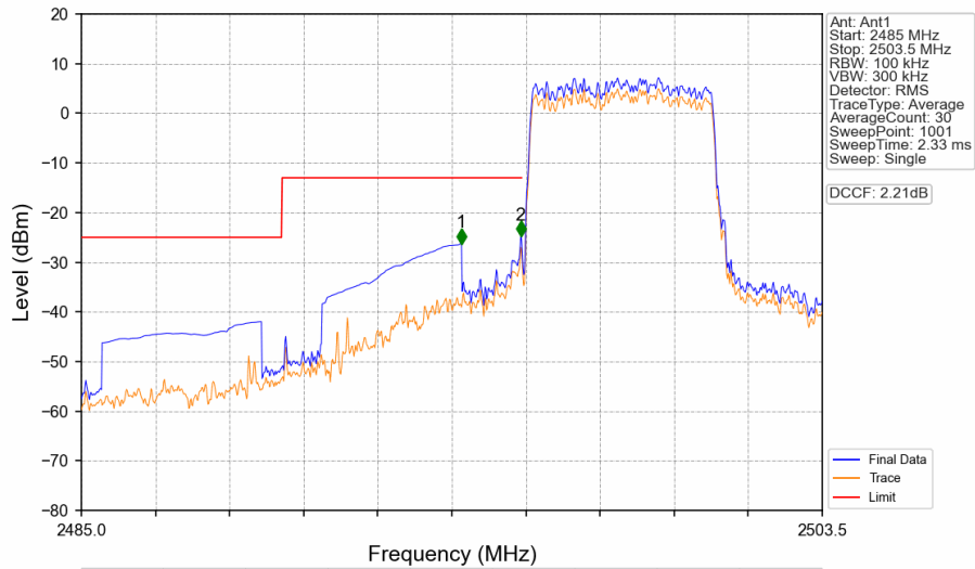
Band41_5MHz_16QAM_LCH_2498.5MHz_RB_25_0_NTNV
