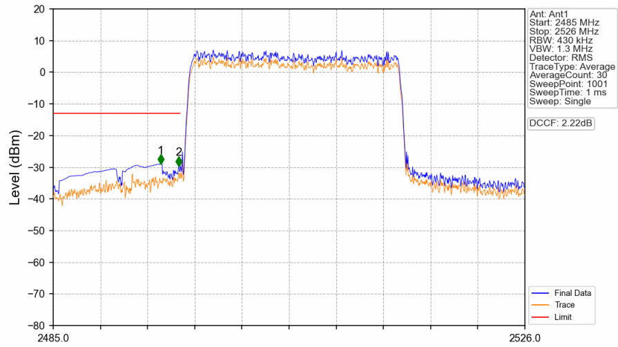
Band41_20MHz_16QAM_LCH_2506MHz_RB_100_0_NTNV
