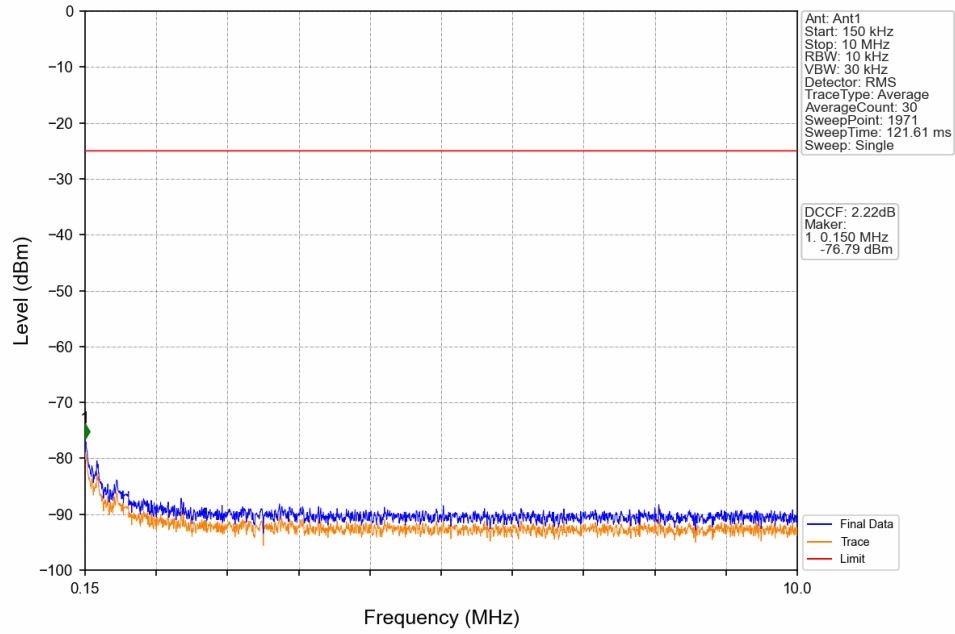
Band41_20MHz_16QAM_LCH_2506MHz_RB_100_0_NTNV
