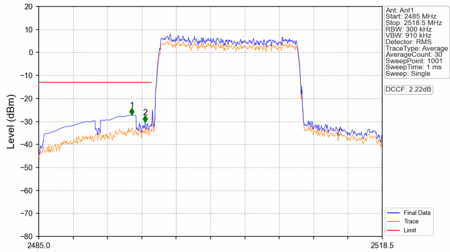
Band41_15MHz_16QAM_LCH_2503.5MHz_RB_75_0_NTNV
