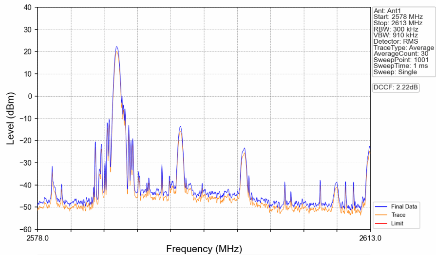
Band41_15MHz_16QAM_MCH_2593MHz_RB_1_0_NTNV
