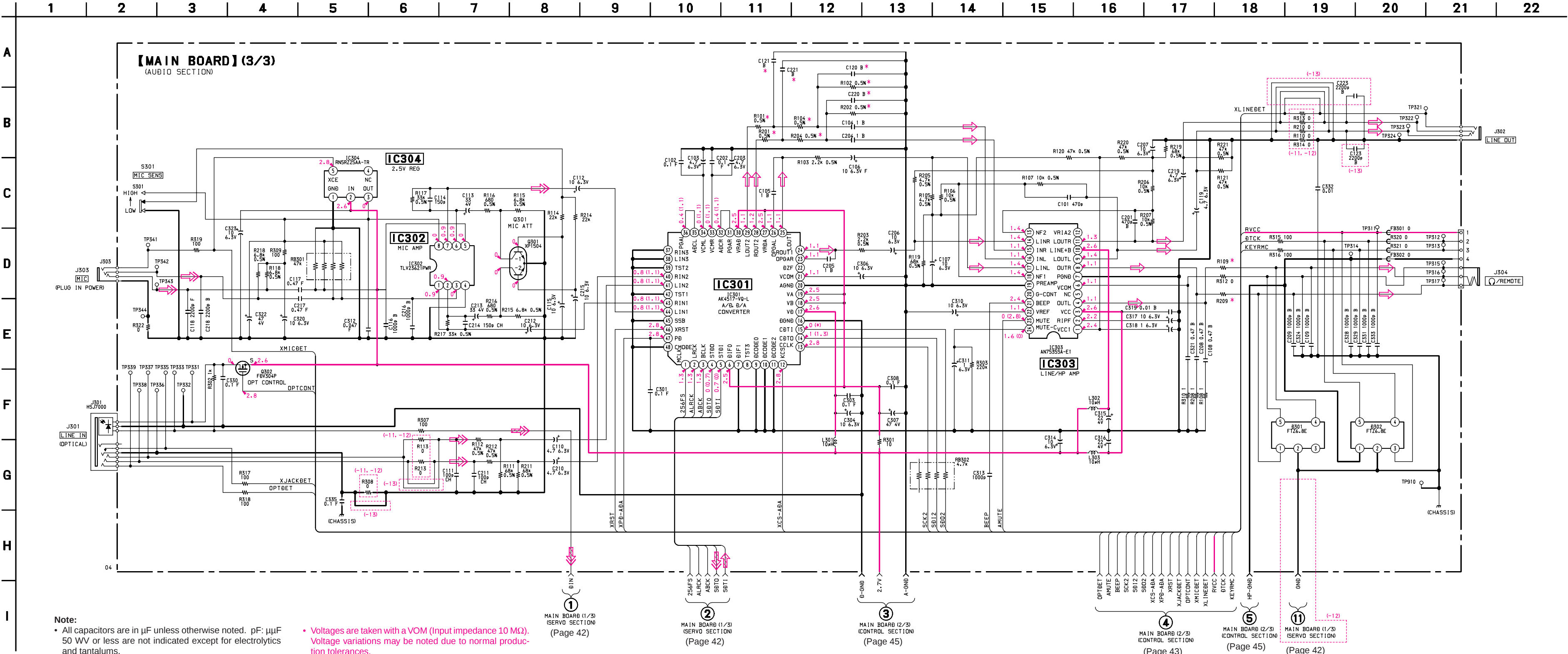
6-10. SCHEMATIC DIAGRAM — MAIN SECTION (3/3) — • Refer to page 49 for IC Block Diagrams.
