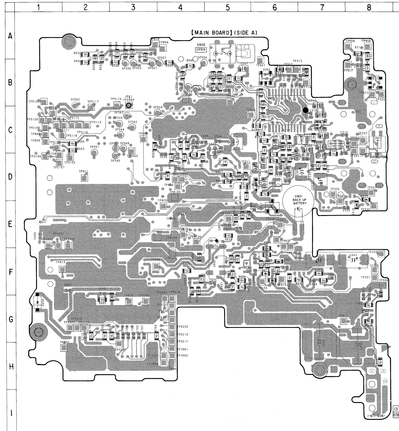
6-7. PRINTED WIRING BOARD (board part number suffix : -13) (All Model)
