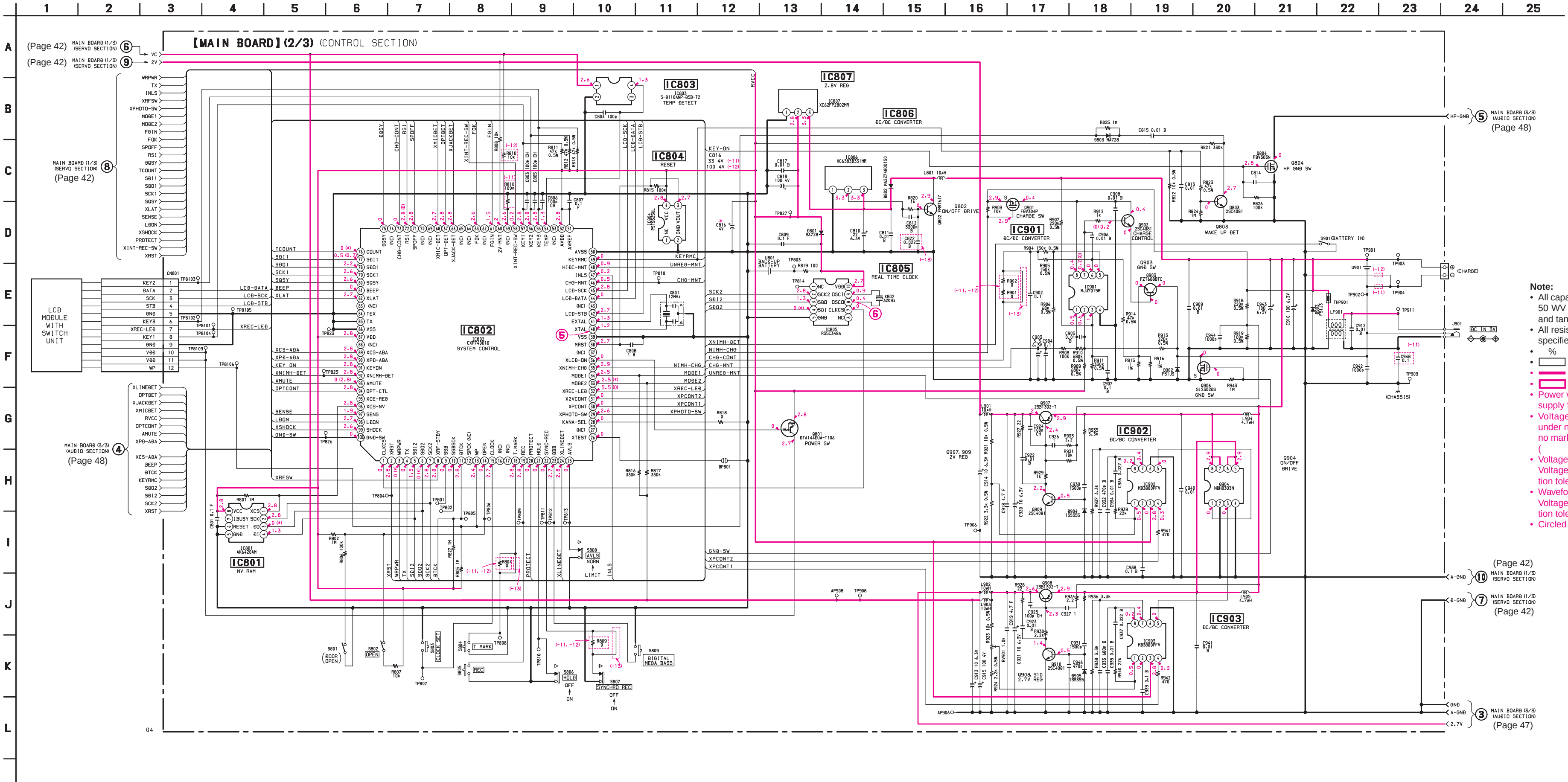
6-9. SCHEMATIC DIAGRAM — MAIN SECTION (2/3) — • Refer to page 49 for IC Block Diagrams.
