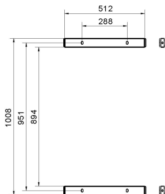
Installation dimensions of fastener strips
