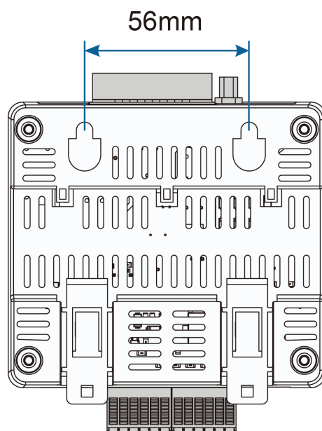
figure 5-1 Mounting Holes
