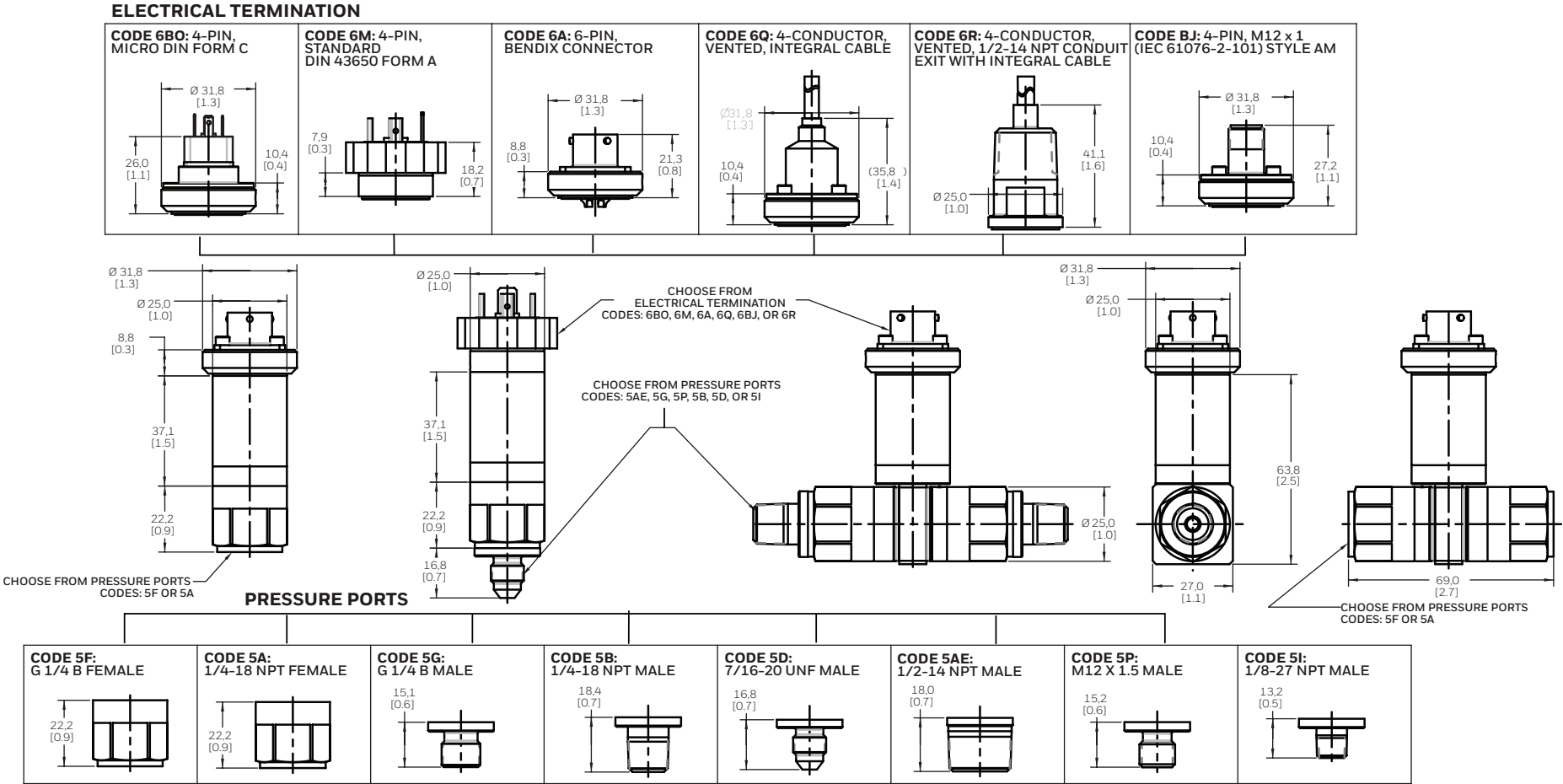
Figure 2. Mounting Dimensions
