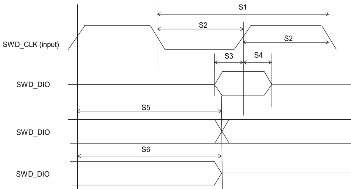
Figure 14. SWD timing
