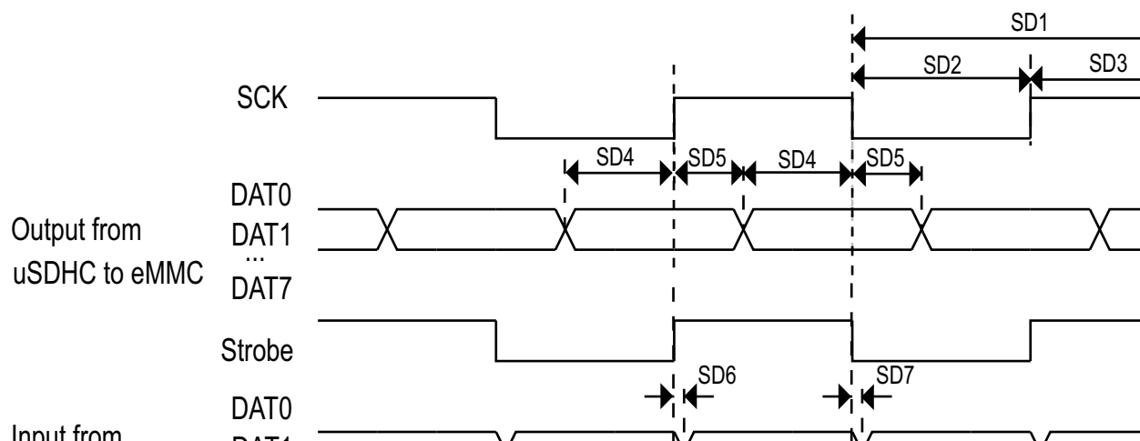
Figure 44. HS400 timing
