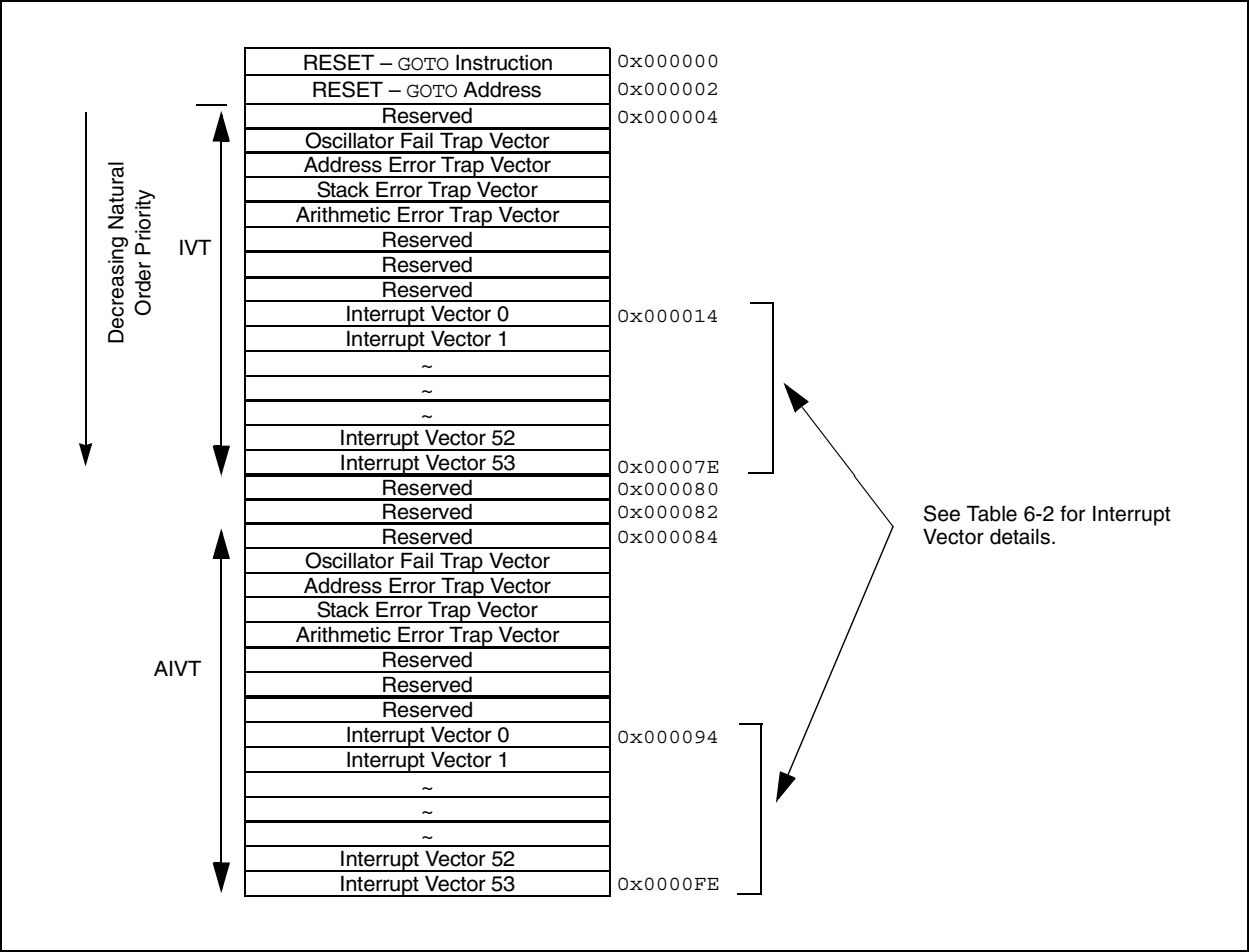
Figure 6-1: Interrupt Vector Table
