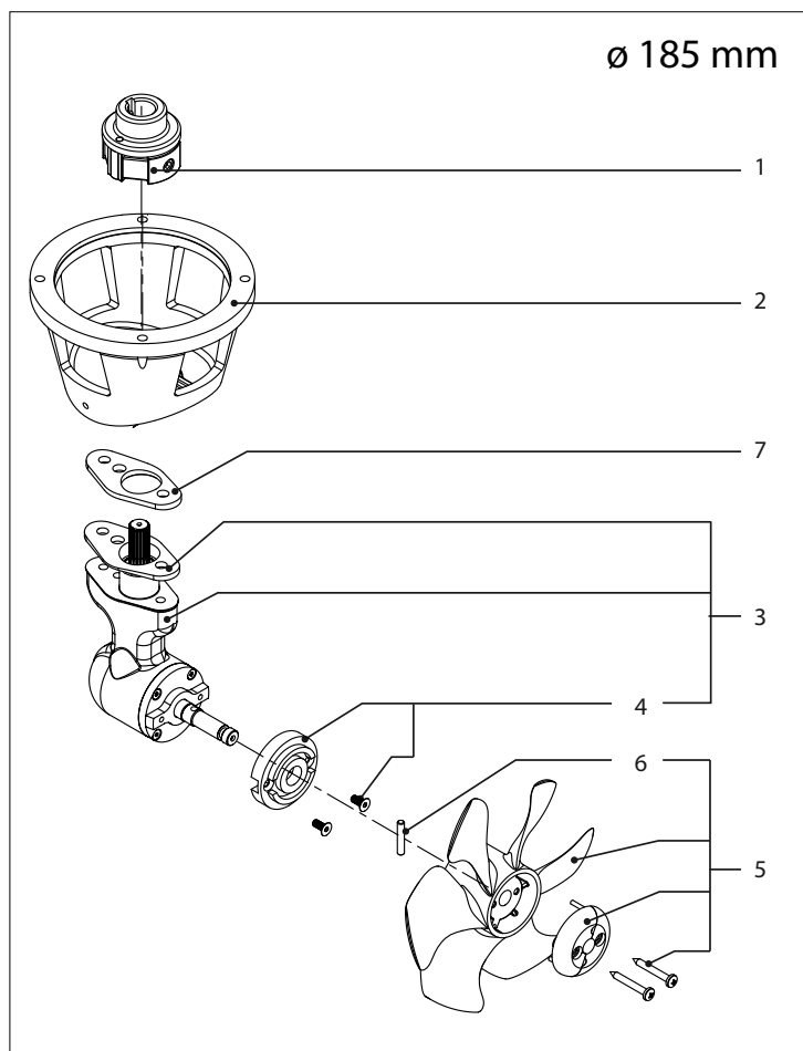
BOWA0651 BOWB076 Service onderdelen, staartstuk BOWA0764 BOWB090 185 mm tunnelbuis BOWA0761 BOWB110 BOWB065 BOWB130
