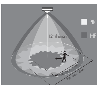
Detection pattern for human
