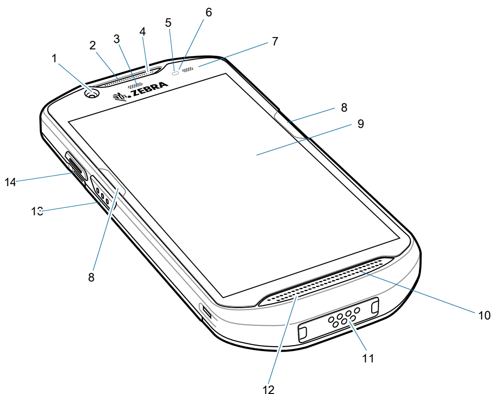
Figure 1 Front View
