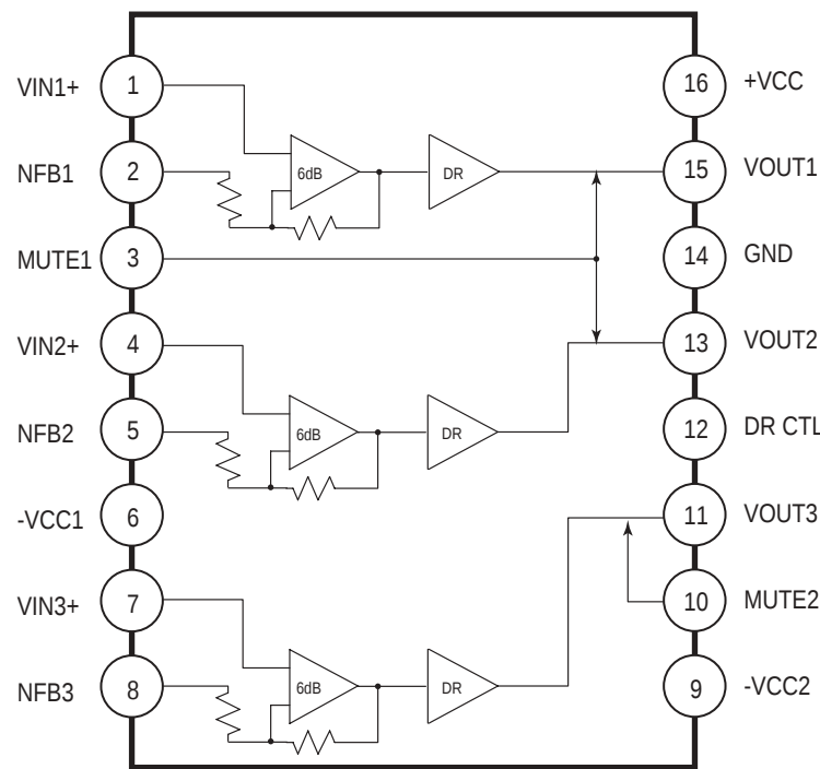
Q2801 LA7106MFP(75 ohm video driver)
