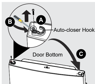
Auto-closer Hook
