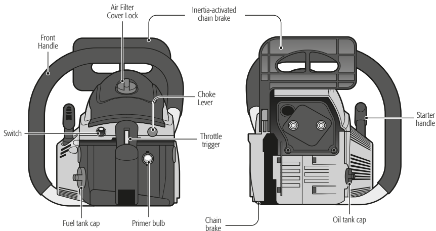
rear view
