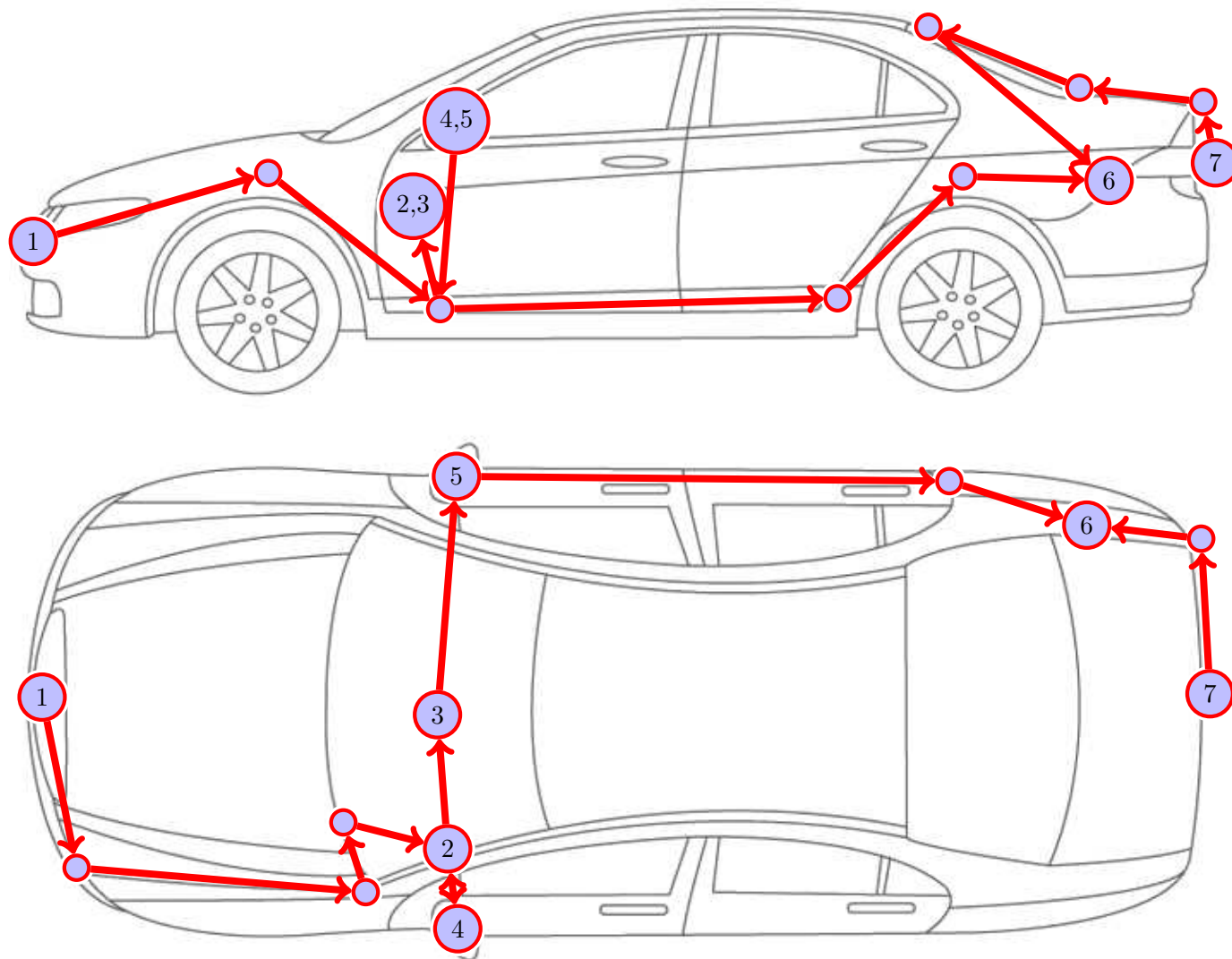
Figure 3: Vehicle overview
