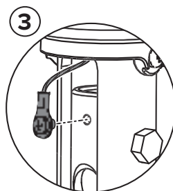
Connect Safety Cable
