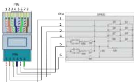
Picture 9: Connection of DRED with PIN communication port
