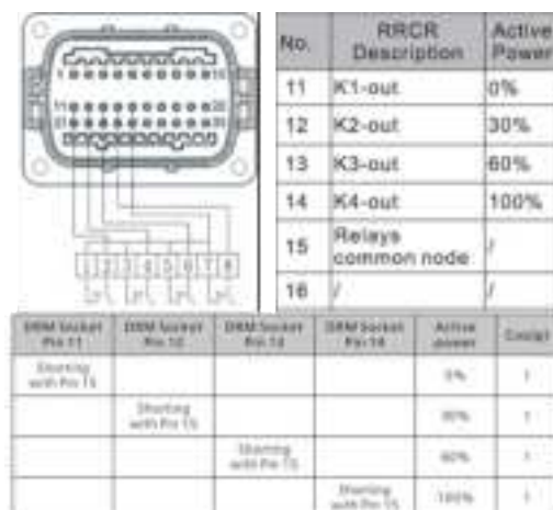
Picture 8: Connection of RRCR with PIN communication port
