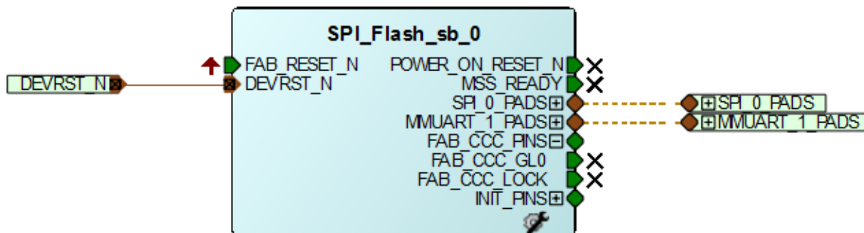
Figure 14 • SPI_Flash SmartDesign
