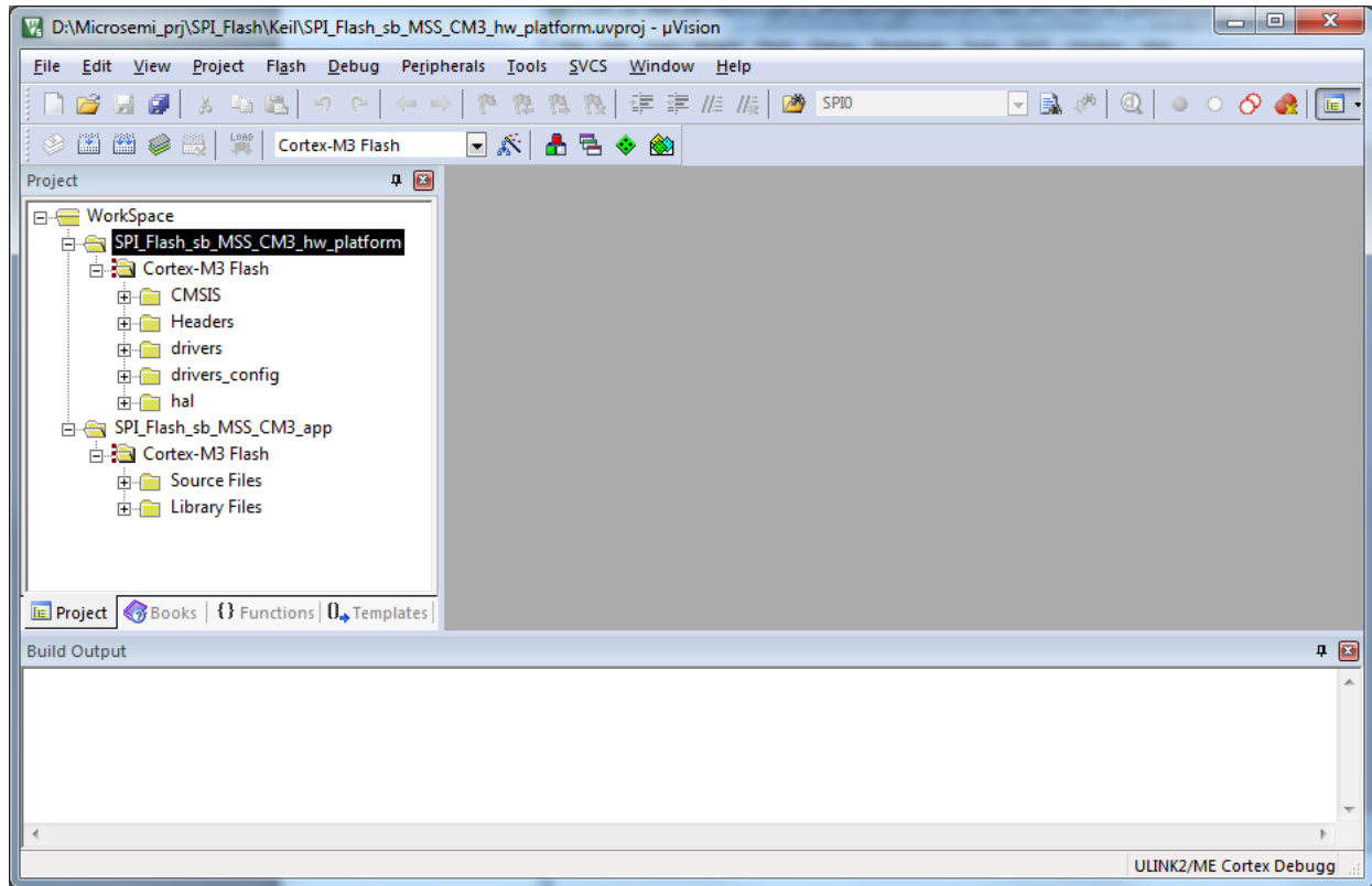
Figure 25 • uVision Workspace
