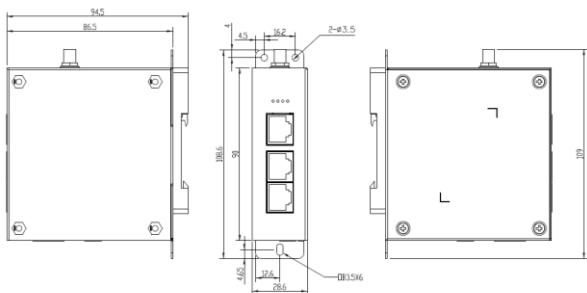
Figure 2-1 Outline dimensions for ICA417 model
